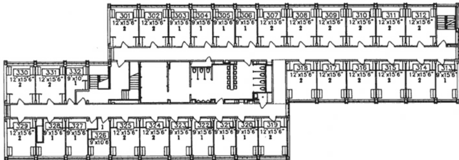
Plantz Hall Third Floor Plan
