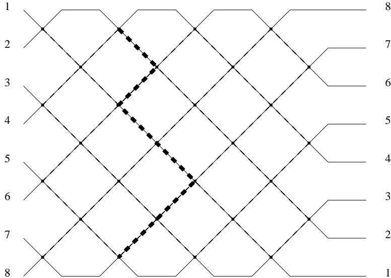
Figure 14: The arrangement for the alternating scheme when n = 8 . The natural partial order is highlighted. An ideal can be identified by its upper boundary.
