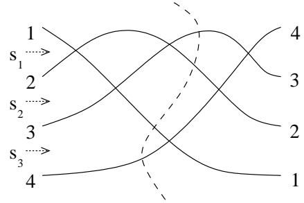
Figure 6: The permutation corresponding to this new pseudoline is 3214
