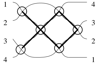
Figure 9: Strings 1, 3 and 4 make an upward pointing triangle
