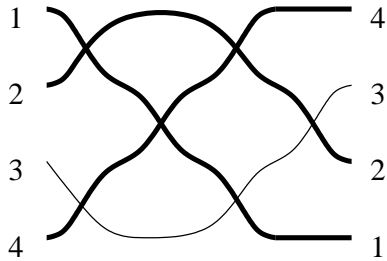
Figure 10: Strings 1, 3 and 4 make a downward pointing triangle
