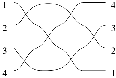
Figure 8: The alternating scheme
