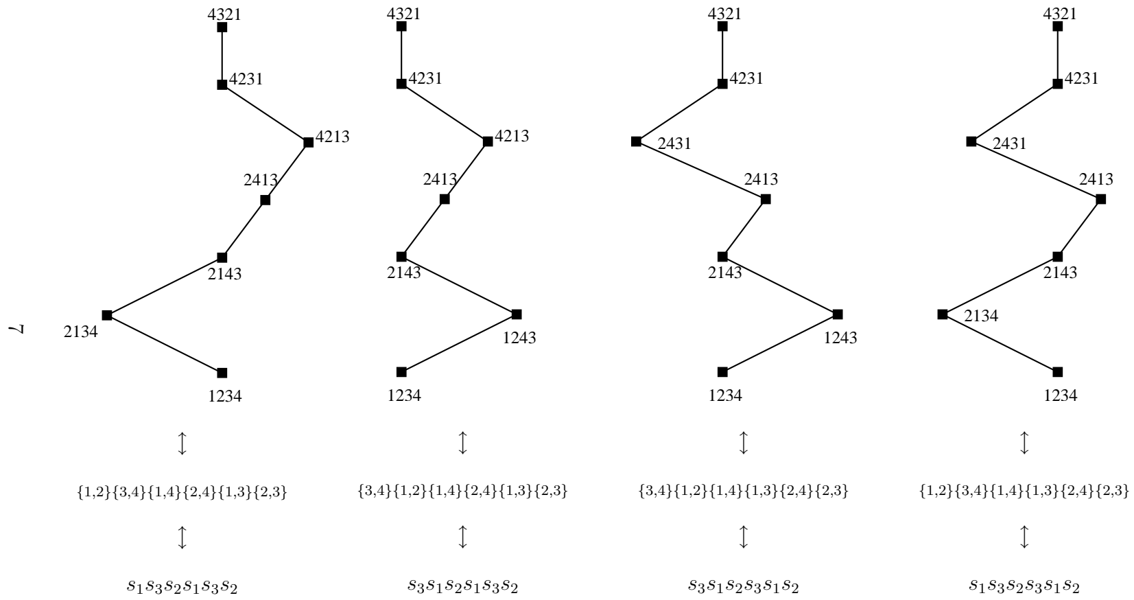
Figure 3: The correspondences among permutations of \binom{[n]}{2} , maximal chains, and maximal reduced decompositions
